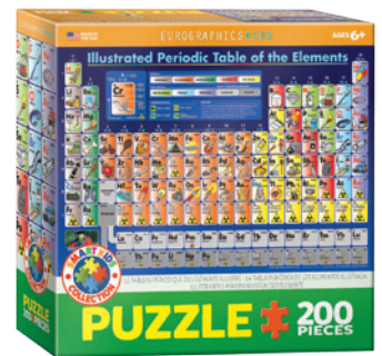
Illustrated Periodic Table
