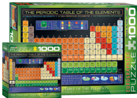
The Periodic Table of the Elements
