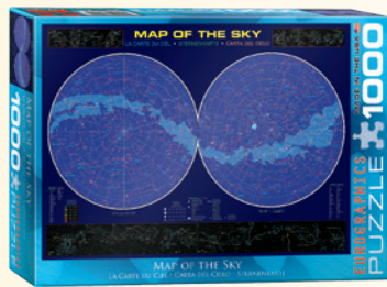
Map of the Sky
